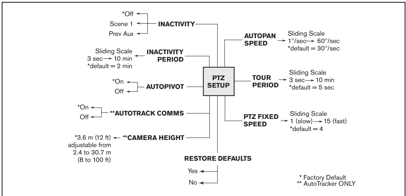
Figure 13C PTZ Setup
