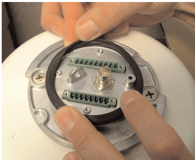
Install Gasket with Lip on Top.
